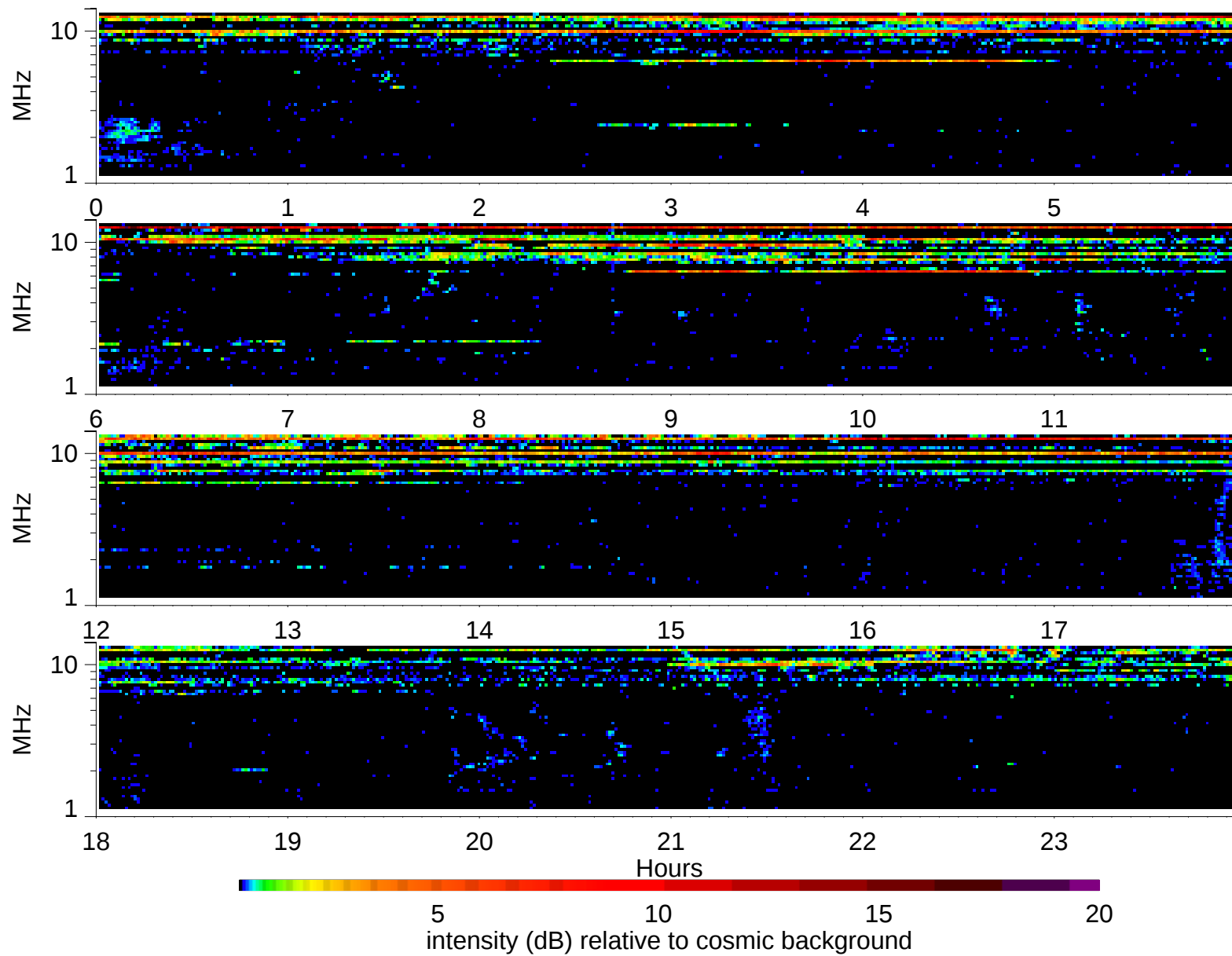
Wind Waves RAD2 receiver: 1995/8/9
