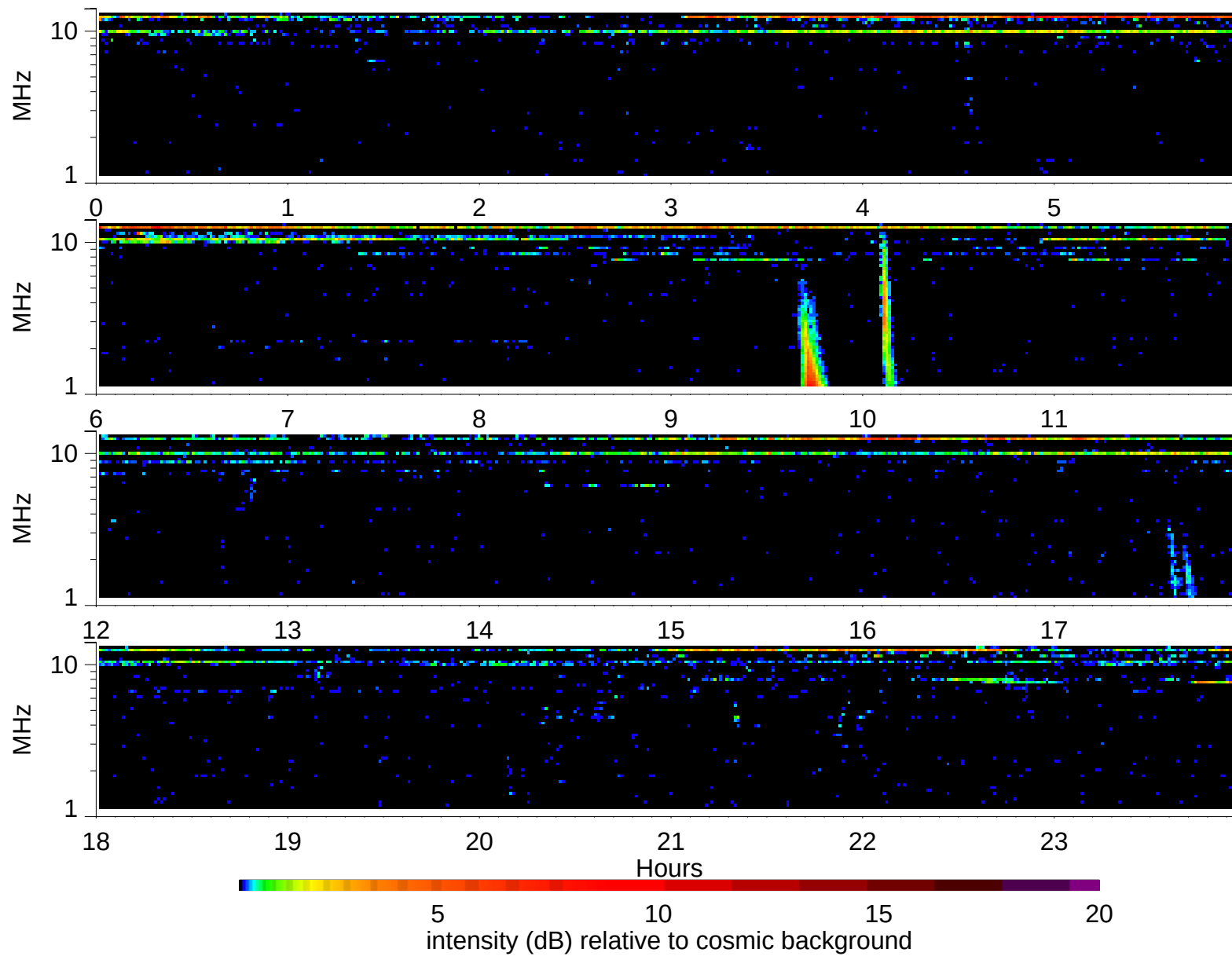
Wind Waves RAD2 receiver: 1995/6/18
