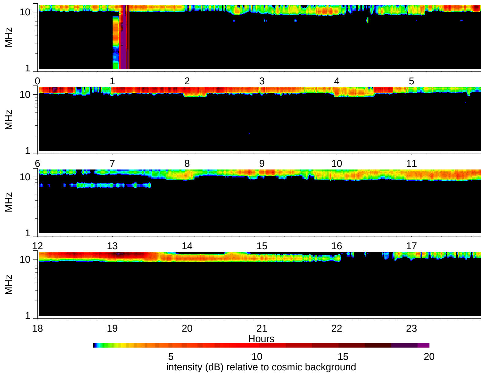
Wind Waves RAD2 receiver: 1995/5/3
