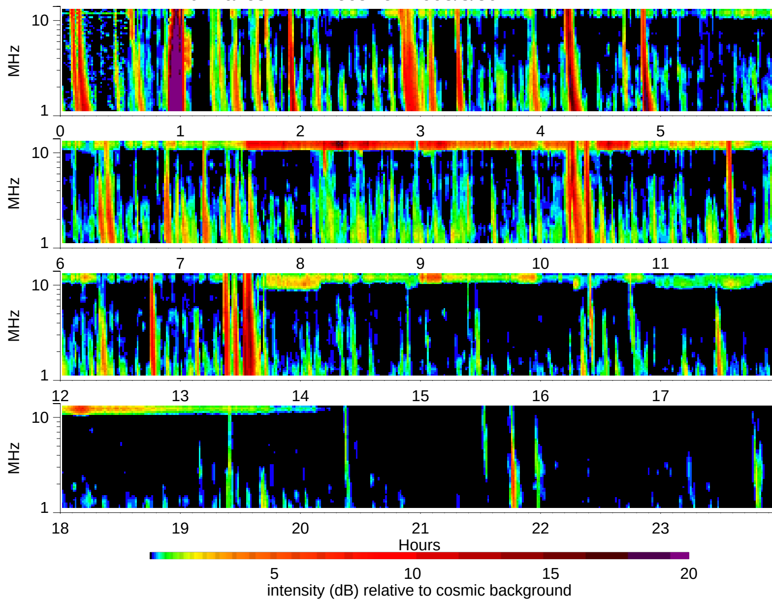
Wind Waves RAD2 receiver: 1995/3/30
