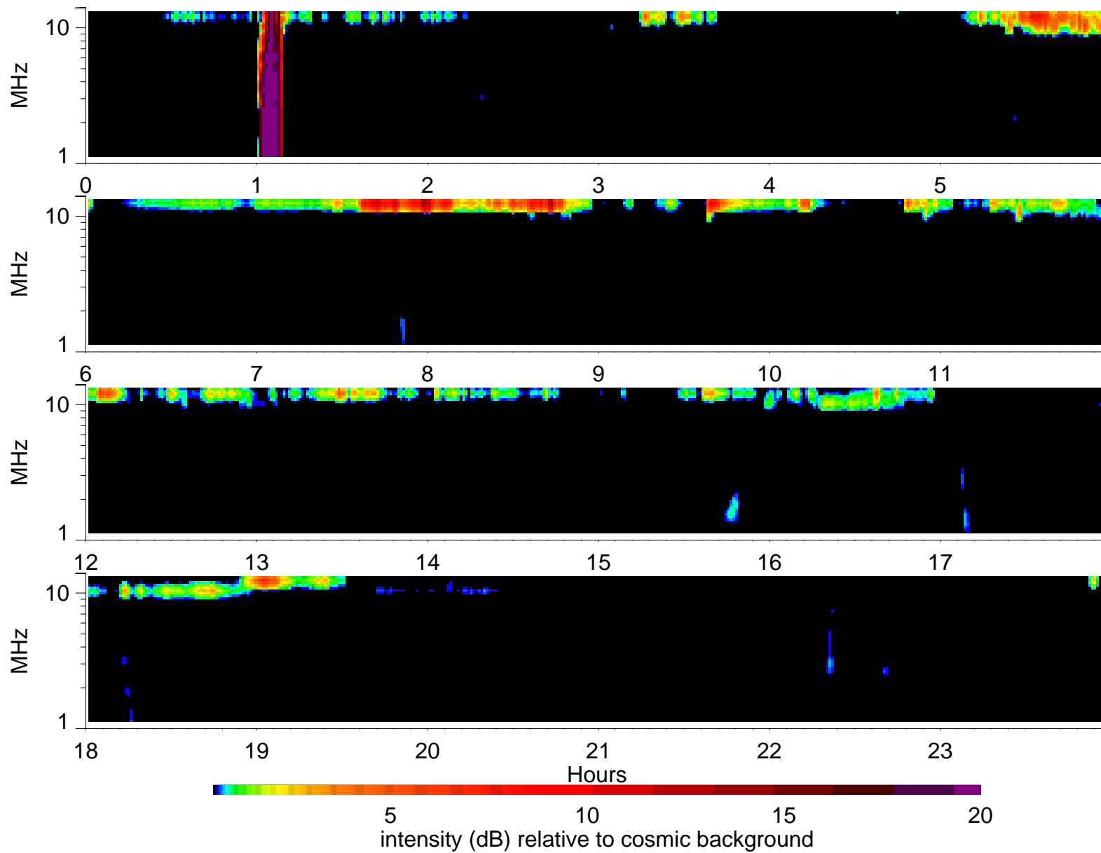
Wind Waves RAD2 receiver: 1995/3/10
