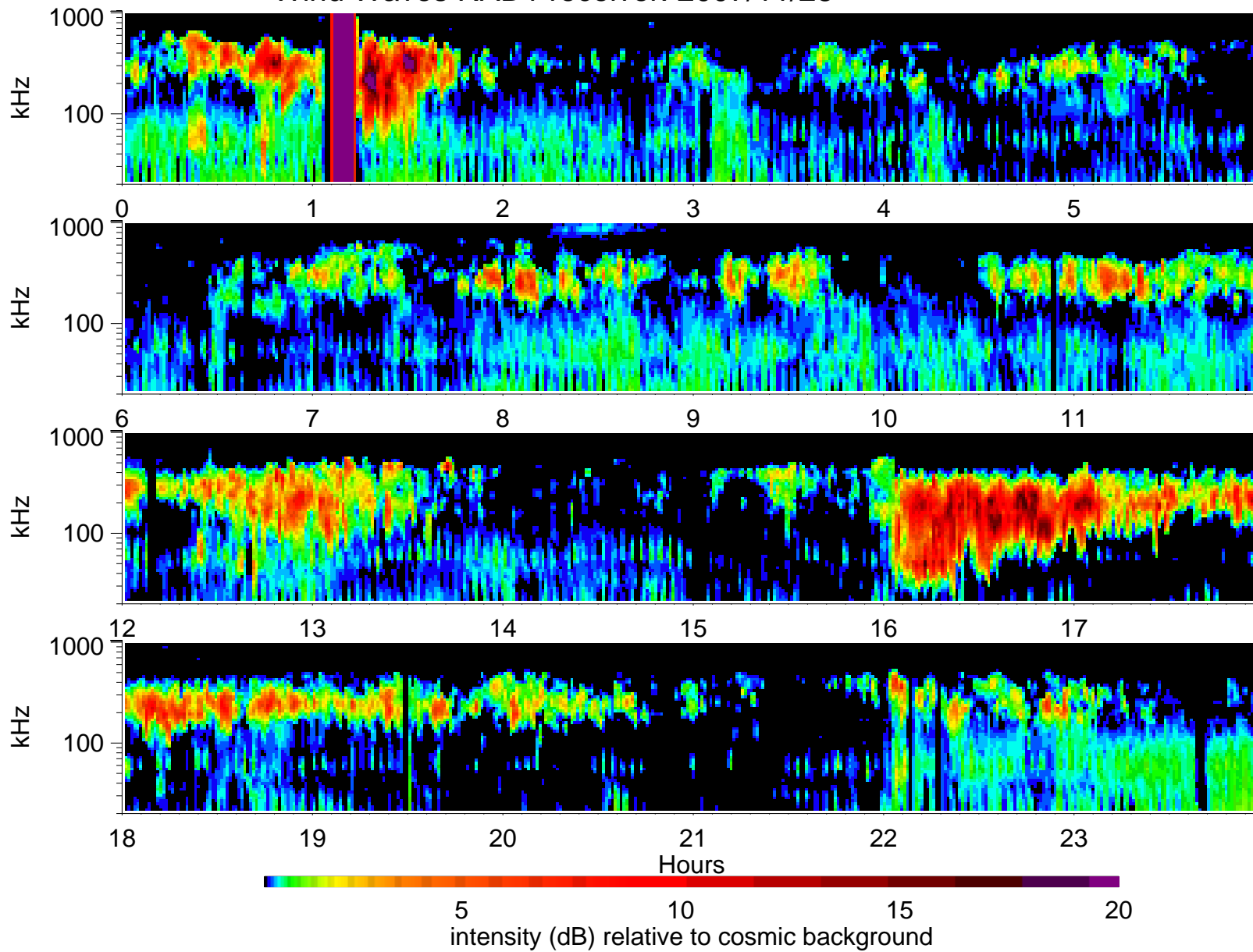
Wind Waves RAD1 receiver: 2007/11/28
