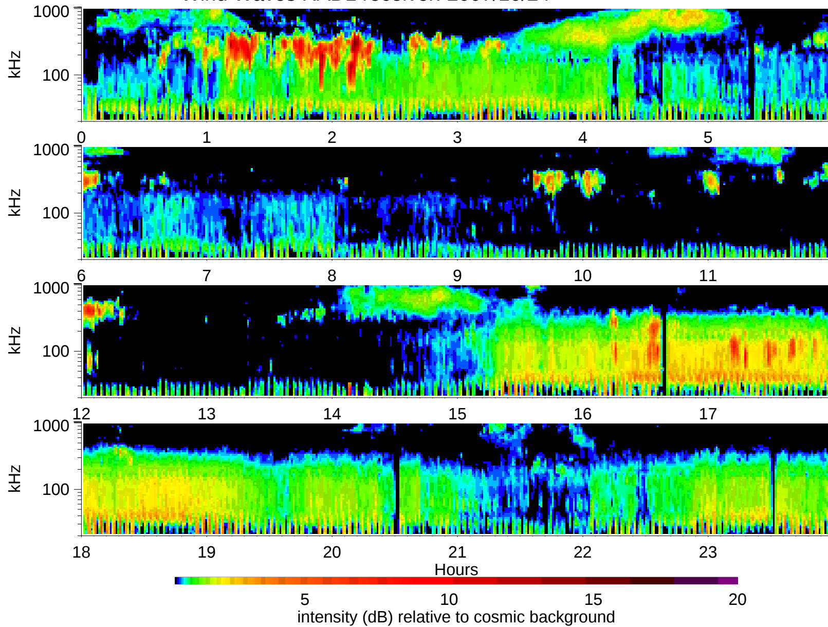
Wind Waves RAD1 receiver: 2007/10/24
