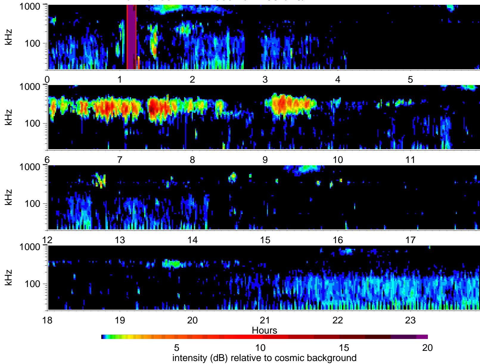
Wind Waves RAD1 receiver: 2007/10/7
