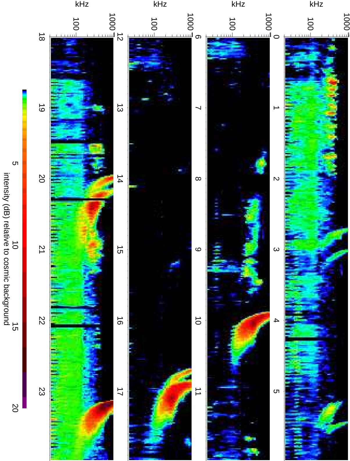
Wind Waves RAD1 receiver: 2007/08/17
