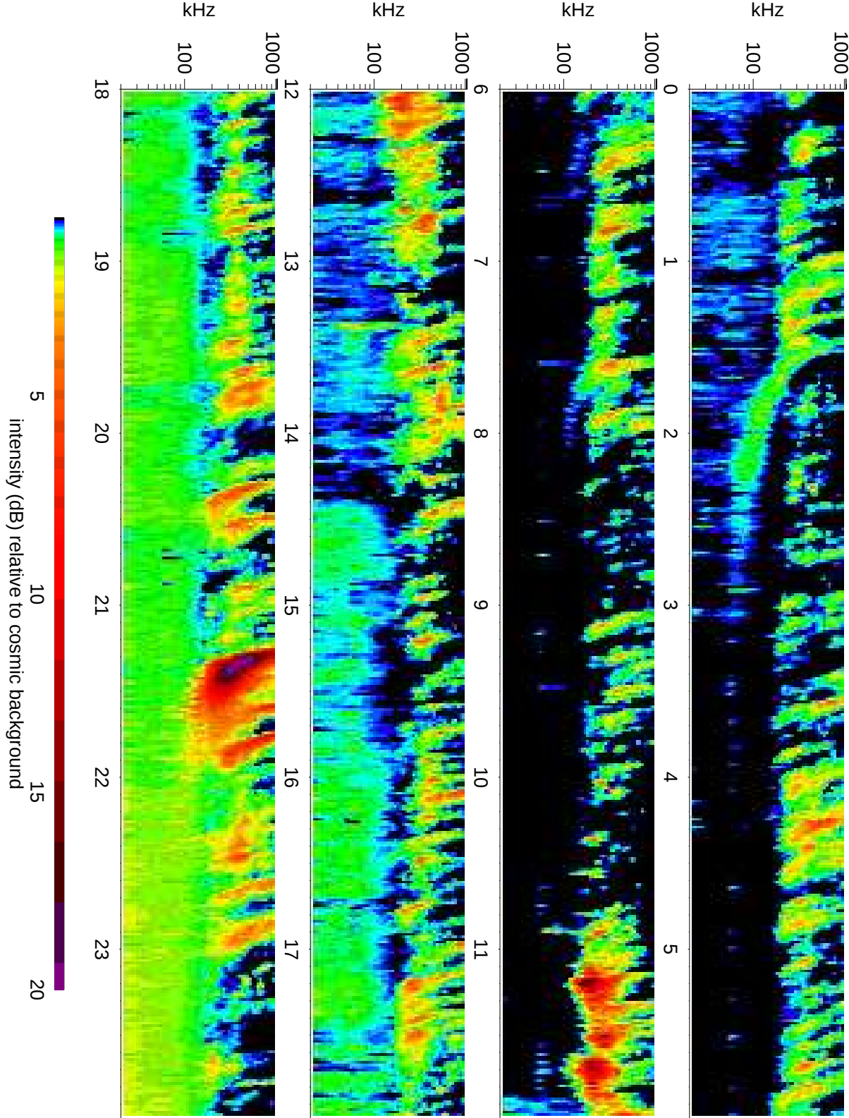
Wind Waves RAD1 receiver: 2007/01/07
