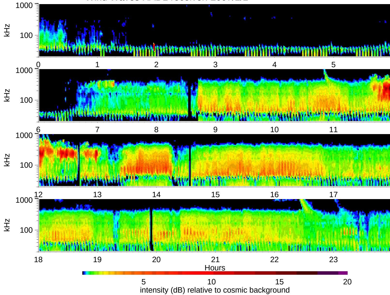
Wind Waves RAD1 receiver: 2007/1/1
