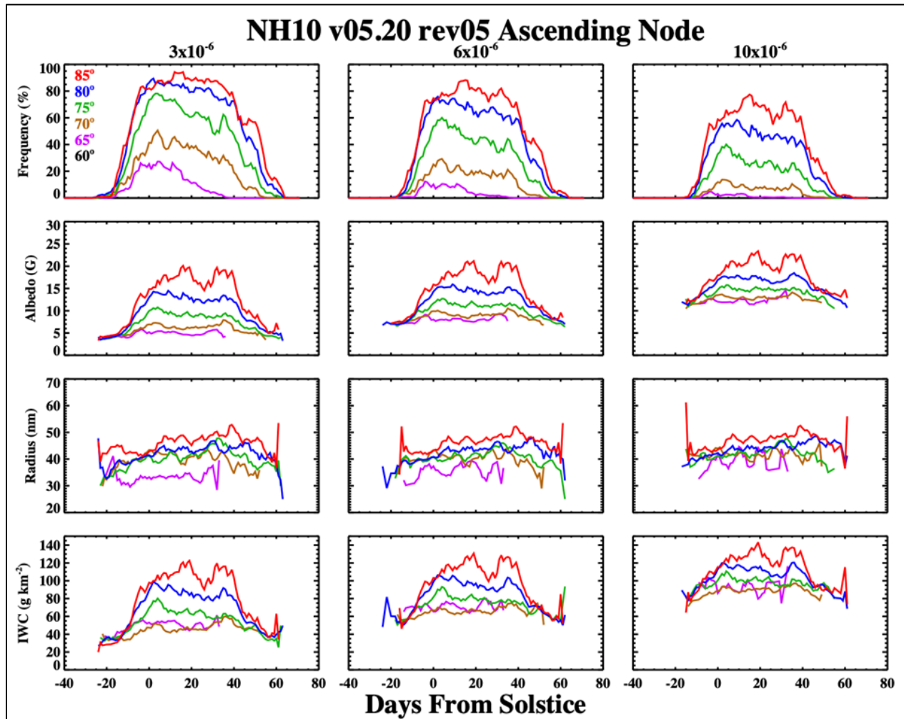
Figure 6. CIPS ascending node PMC frequencies (top), albedo (row 2), radius (row 3), and IWC (bottom) for the NH 2010 season. The columns show the results for measurements that include only those clouds brighter than 3 \times 10^{-6} \text{ sr}^{-1} (left), 6 \times 10^{-6} \text{ sr}^{-1} (middle) and 10 \times 10^{-6} \text{ sr}^{-1} (right). Colors correspond to latitude, as denoted by the labels in the top left panel. The plots were made with level 3C data.
