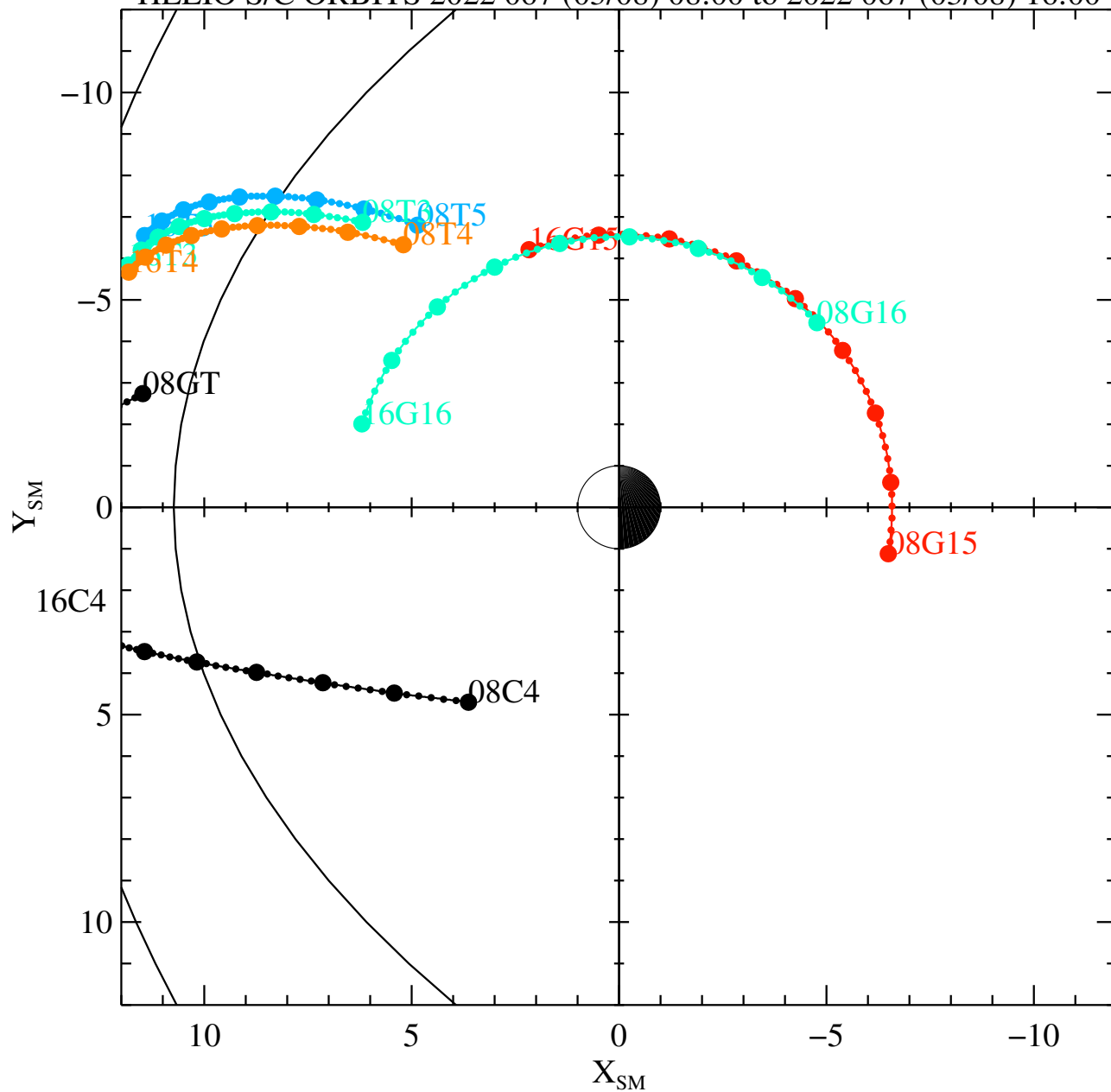
HELIO S/C ORBITS 2022 067 (03/08) 08:00 to 2022 067 (03/08) 16:00
