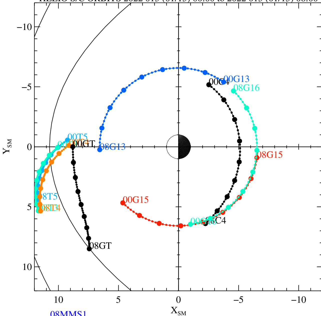
HELIO S/C ORBITS 2022 015 (01/15) 00:00 to 2022 015 (01/15) 08:00
