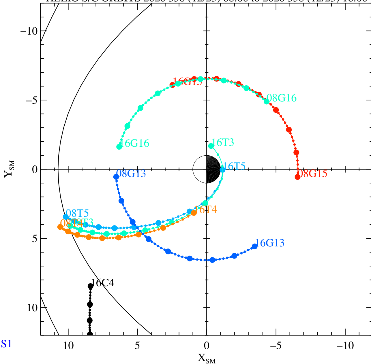
HELIO S/C ORBITS 2020 358 (12/23) 08:00 to 2020 358 (12/23) 16:00
