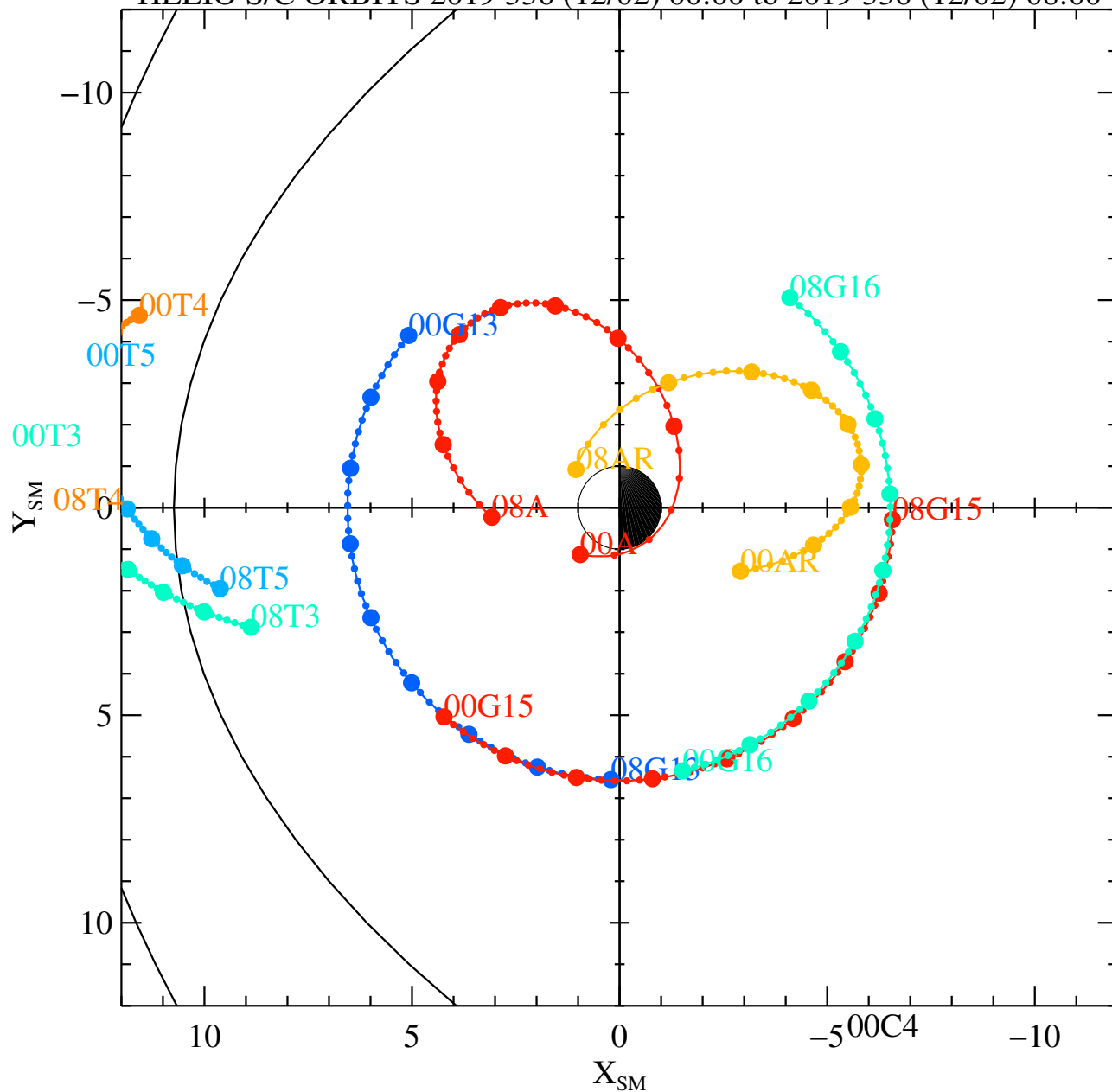
HELIO S/C ORBITS 2019 336 (12/02) 00:00 to 2019 336 (12/02) 08:00
