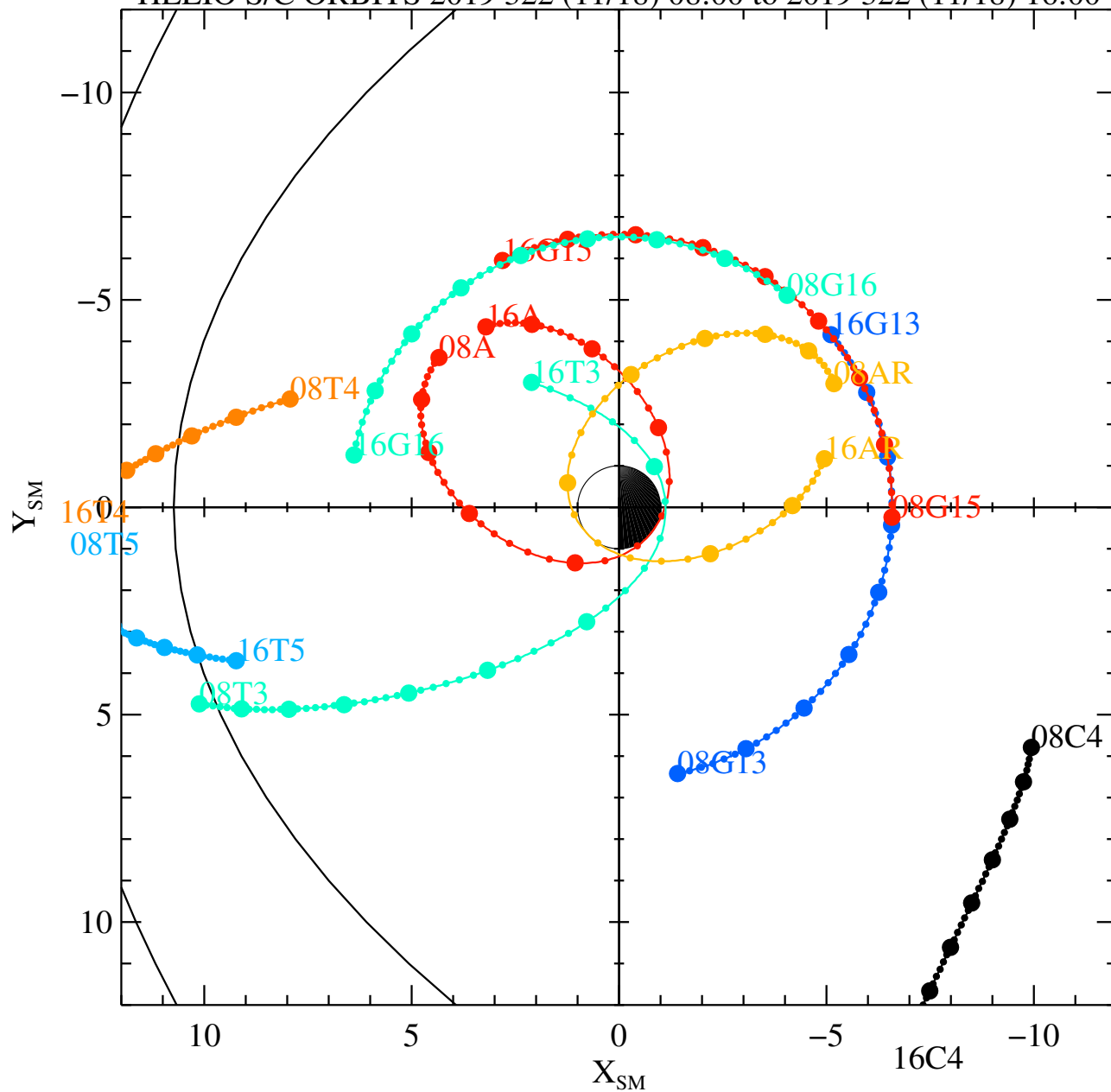
HELIO S/C ORBITS 2019 322 (11/18) 08:00 to 2019 322 (11/18) 16:00
