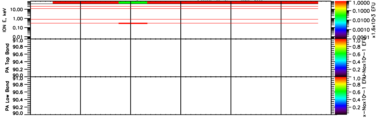
THEMIS-D 2007-10-4-13:00, Ion Spectrograms &amp; Moments.
