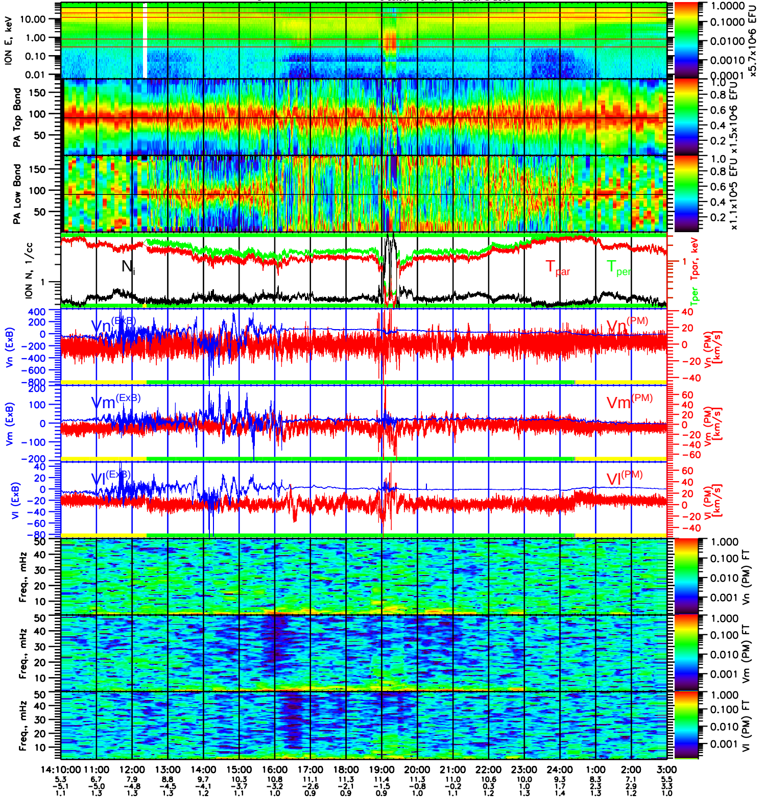
THEMIS-D 2009-10-14, Ion Spectrograms &amp; Moments.
