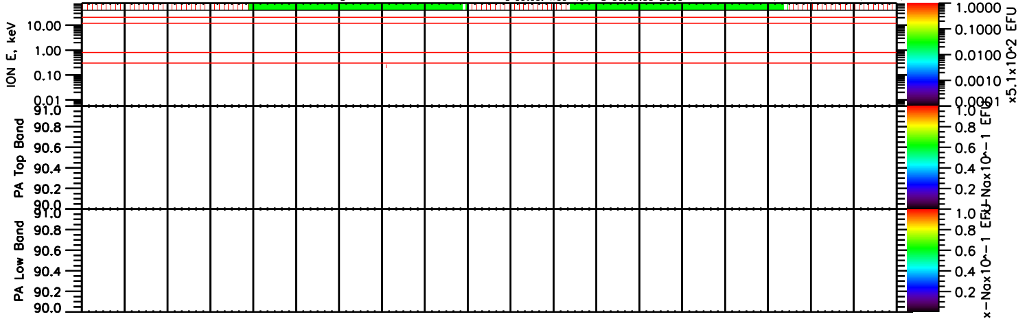
THEMIS-D 2007-10-7, Ion Spectrograms &amp; Moments.
