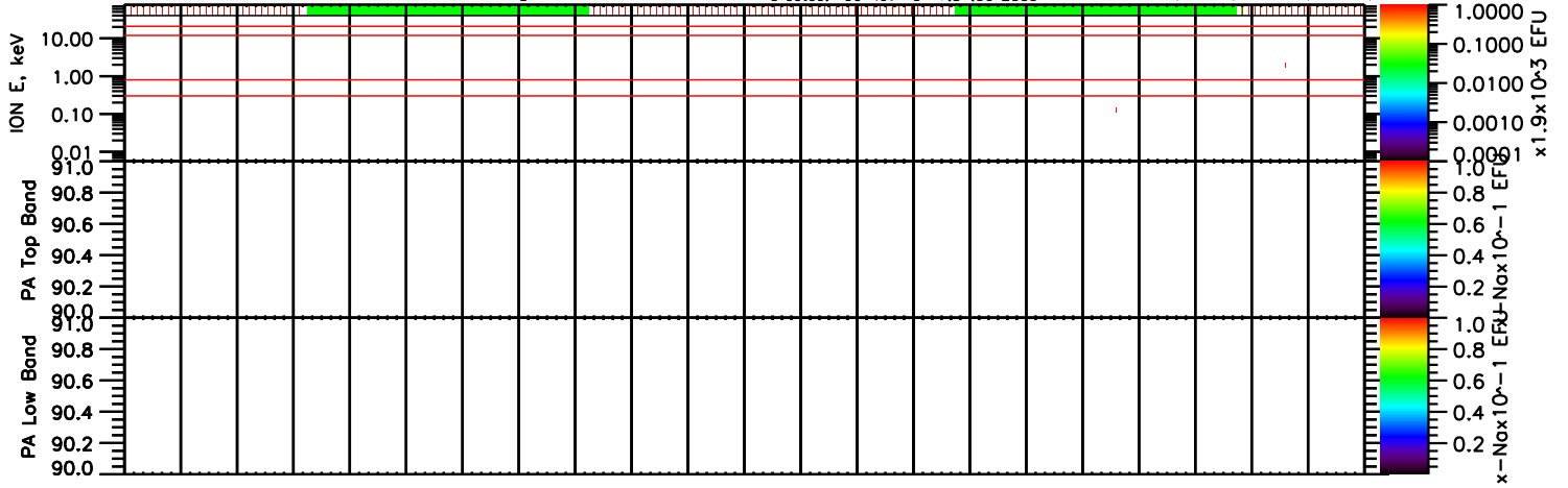
THEMIS-D 2007-10-2, Ion Spectrograms & Moments.
