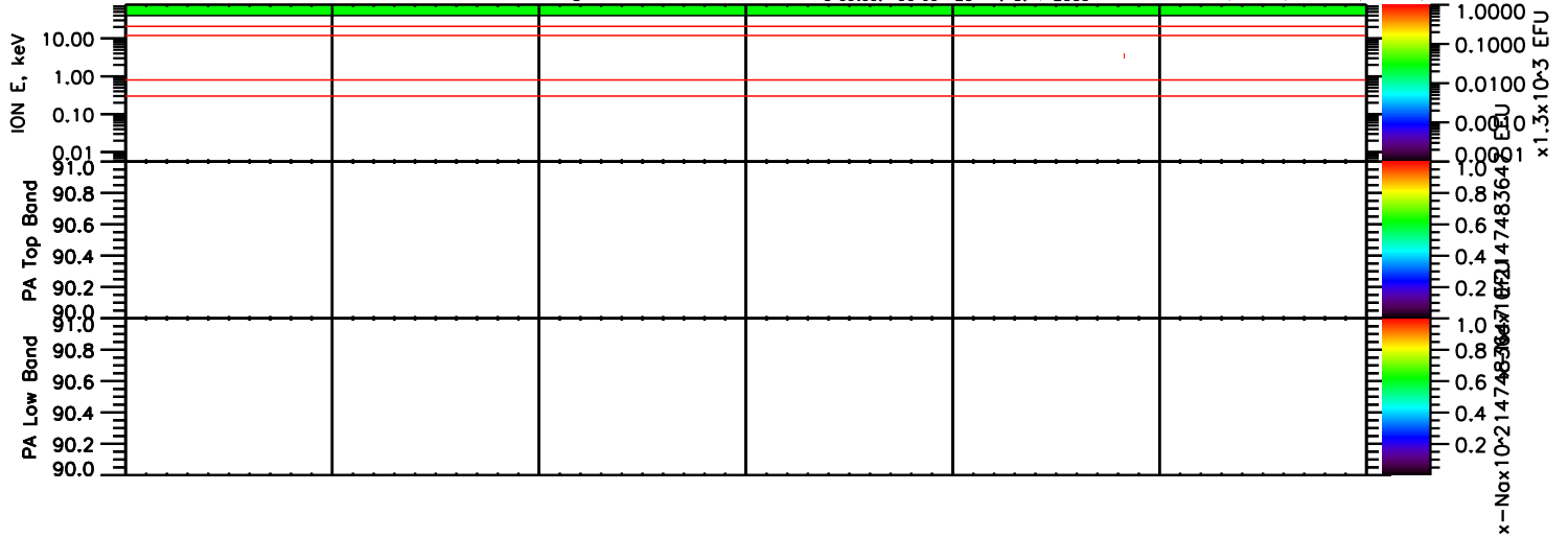
THEMIS-C 2007-10-20-01:00, Ion Spectrograms &amp; Moments.
