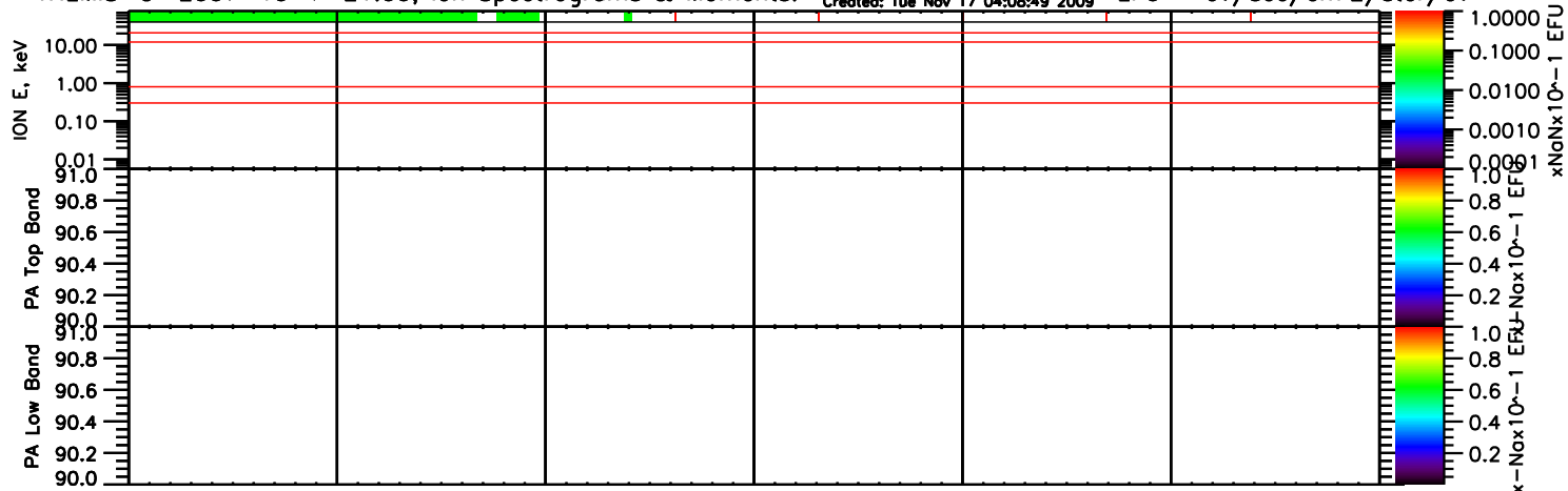
THEMIS-C 2007-10-7-21:00, Ion Spectrograms &amp; Moments.
