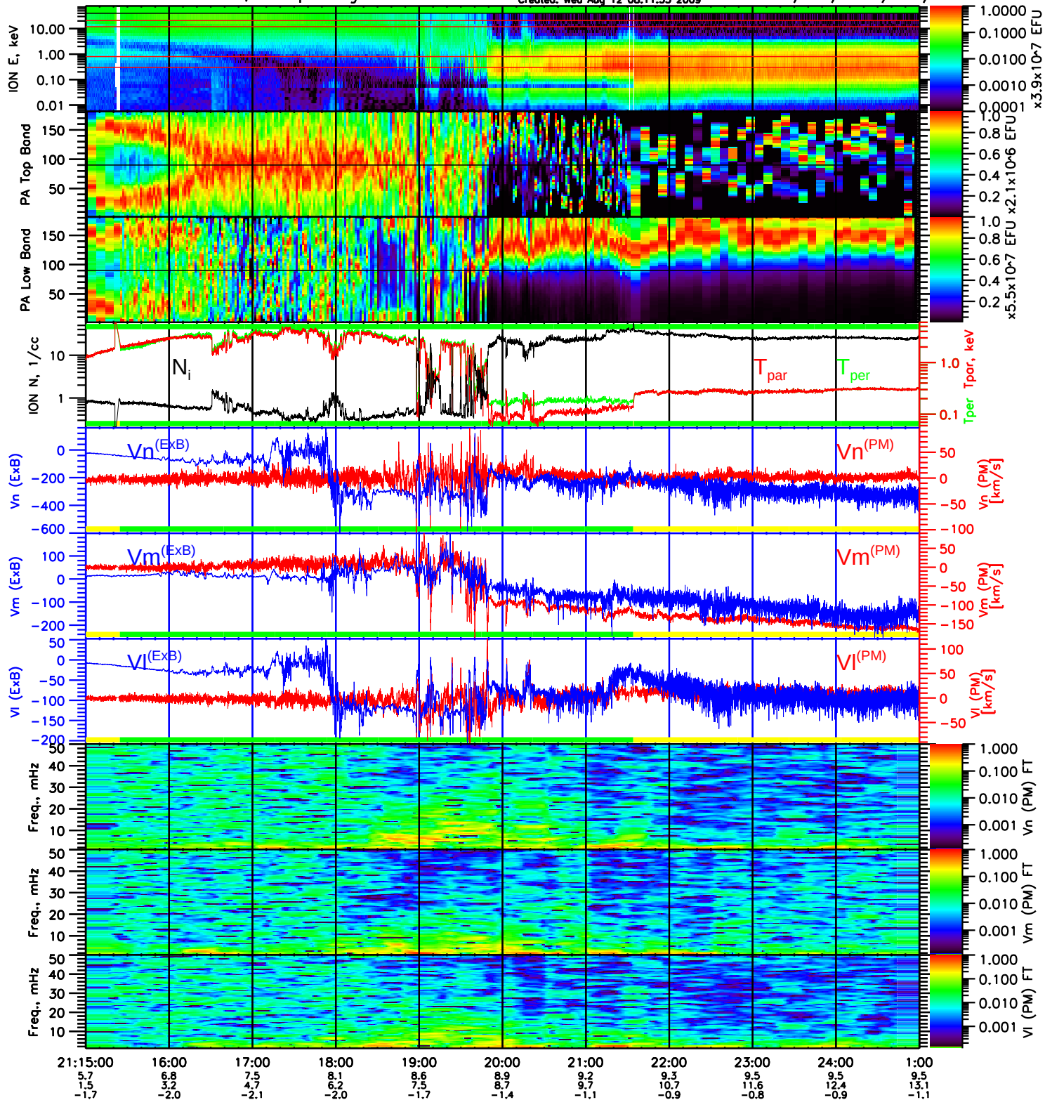
THEMIS-C 2009-06-21, Ion Spectrograms &amp; Moments.
