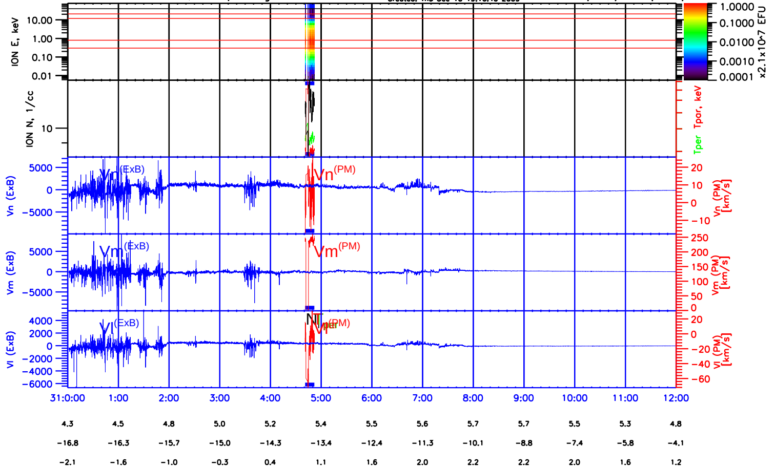
THEMIS-C 2007-10-31, Ion Spectrograms &amp; Moments.
