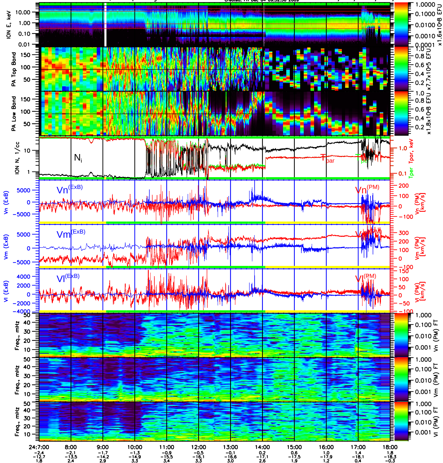
THEMIS-C 2007-10-24, Ion Spectrograms &amp; Moments.
