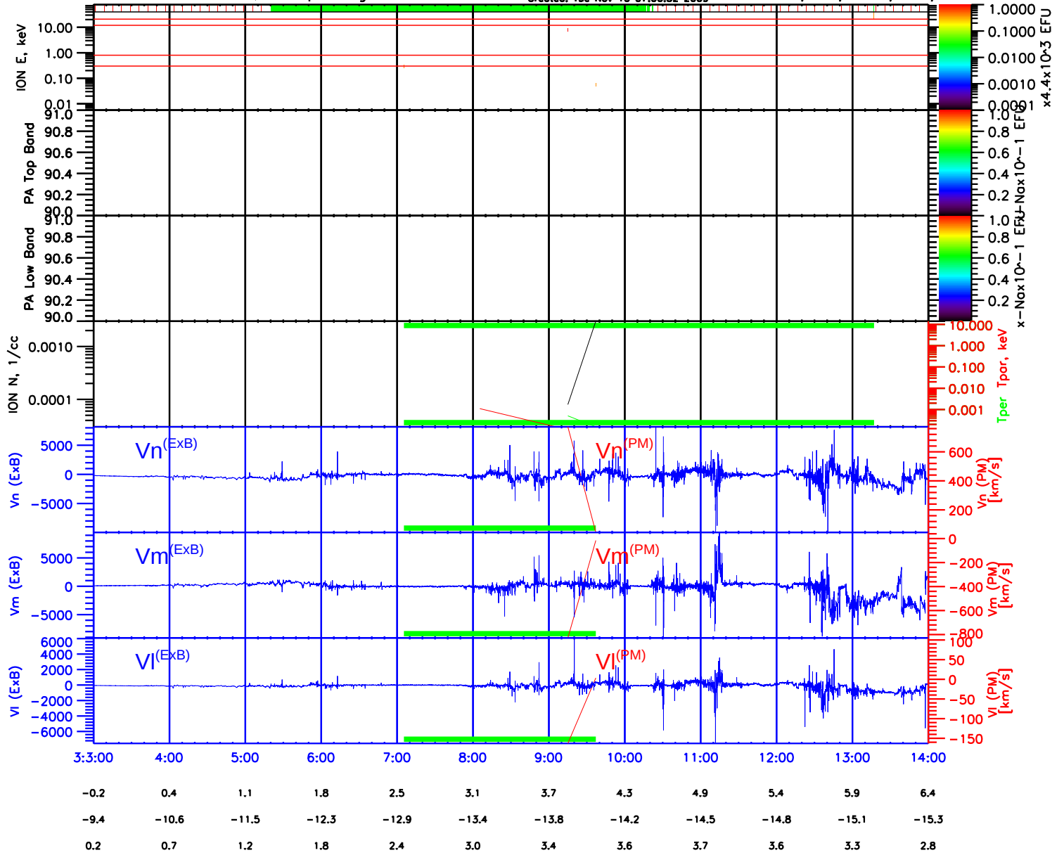
THEMIS-C 2007-10-3, Ion Spectrograms &amp; Moments.
