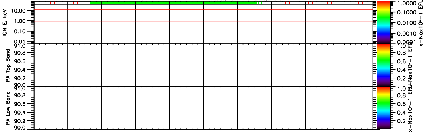
THEMIS-C 2007-10-1, Ion Spectrograms & Moments.
