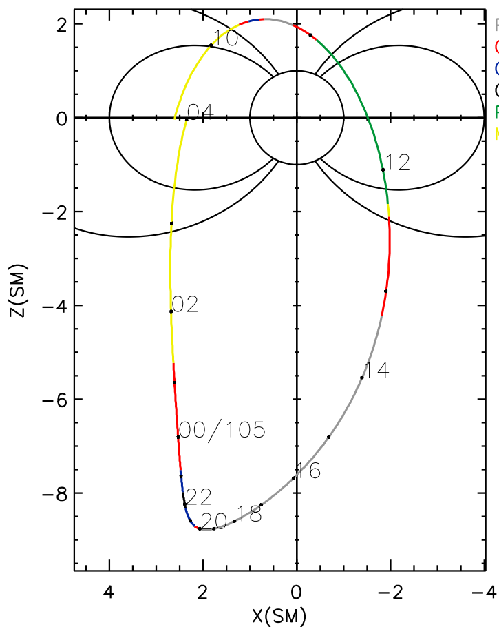
POLAR orbit 2007 104 (04/14) 09:09 UT to 2007 105 (04/15) 04:00 UT
