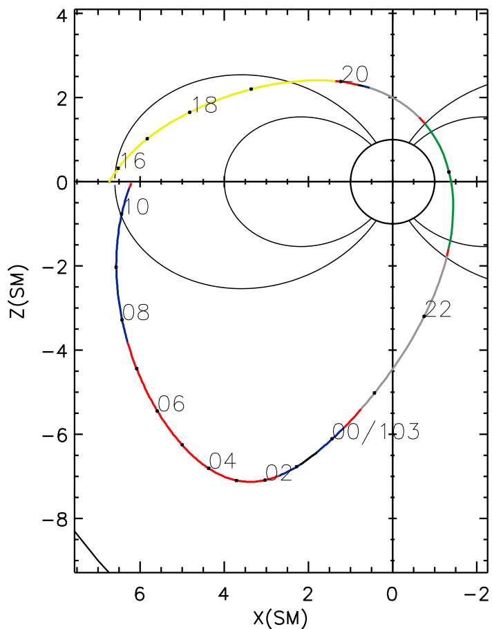
POLAR orbit 2004 102 (04/11) 15:33 UT to 2004 103 (04/12) 10:36 UT
