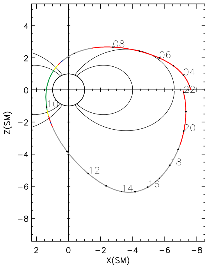
POLAR orbit 2003 289 (10/16) 02:39 UT to 2003 289 (10/16) 22:06 UT
