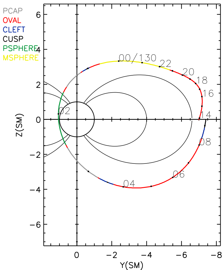
POLAR orbit 2002 129 (05/09) 13:51 UT to 2002 130 (05/10) 09:18 UT
