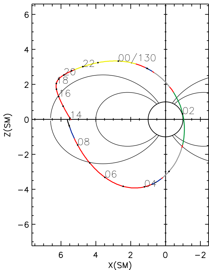
POLAR orbit 2002 129 (05/09) 13:51 UT to 2002 130 (05/10) 09:18 UT
