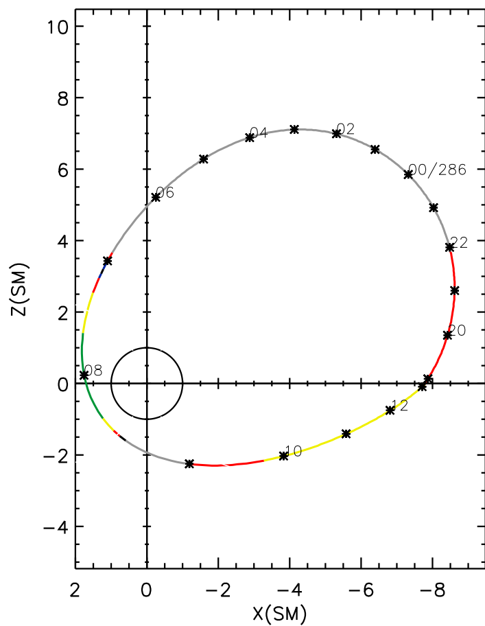
POLAR orbit 2000 285 (10/11) 18:51 UT to 2000 286 (10/12) 13:06 UT
