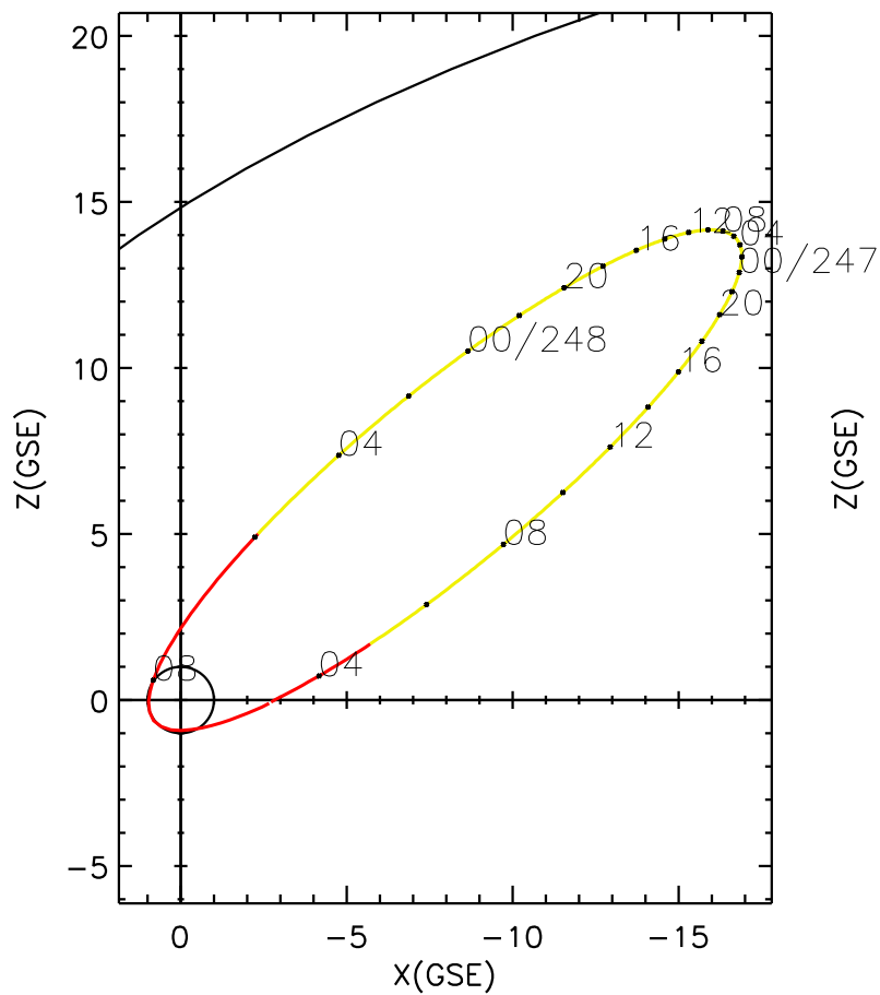
CLUSTER 2 orbit 2024 246 (09/02) 03:21 UT to 2024 248 (09/04) 09:26 UT
