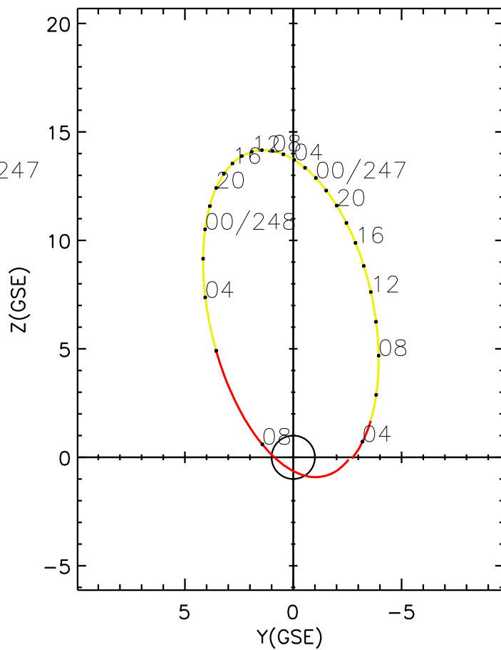
CLUSTER 2 orbit 2024 246 (09/02) 03:21 UT to 2024 248 (09/04) 09:26 UT
