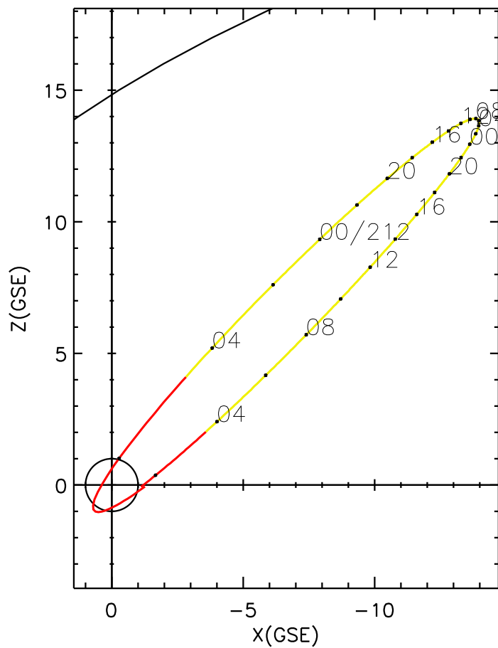
CLUSTER 2 orbit 2024 210 (07/28) 01:36 UT to 2024 212 (07/30) 07:51 UT
