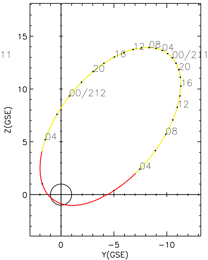
CLUSTER 2 orbit 2024 210 (07/28) 01:36 UT to 2024 212 (07/30) 07:51 UT
