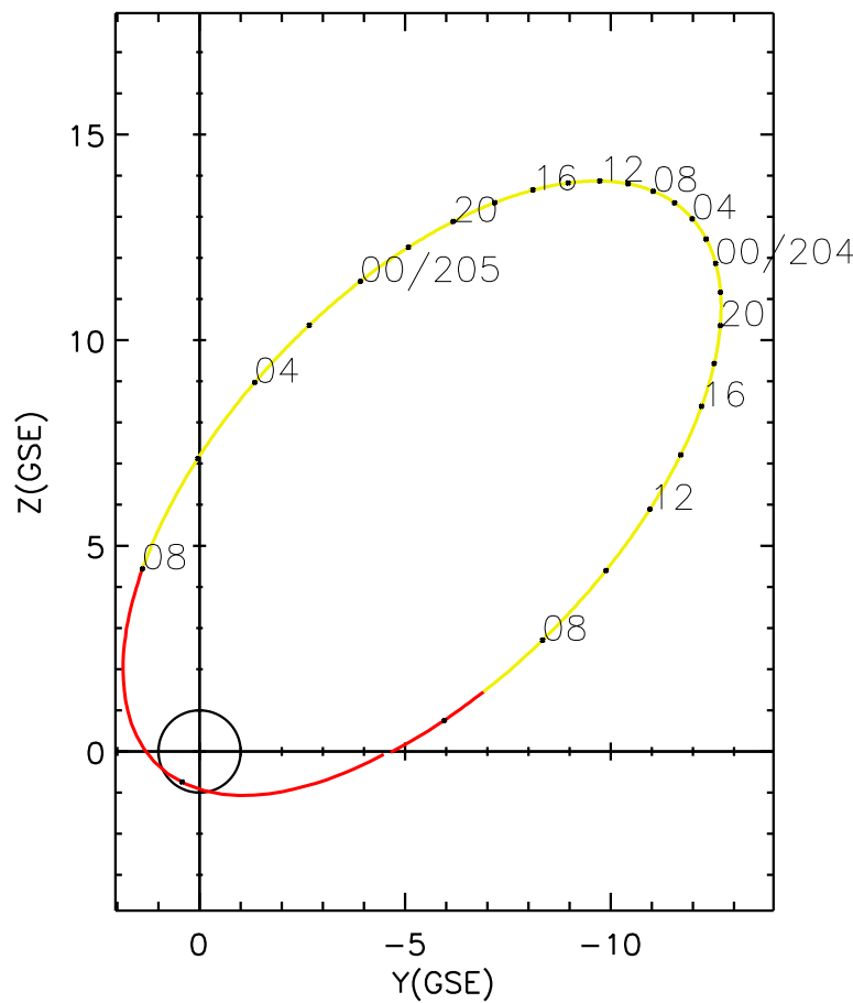
CLUSTER 2 orbit 2024 203 (07/21) 05:16 UT to 2024 205 (07/23) 11:26 UT
