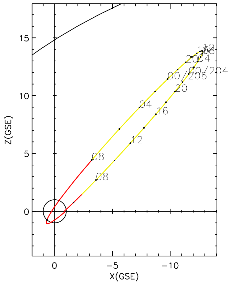
CLUSTER 2 orbit 2024 203 (07/21) 05:16 UT to 2024 205 (07/23) 11:26 UT
