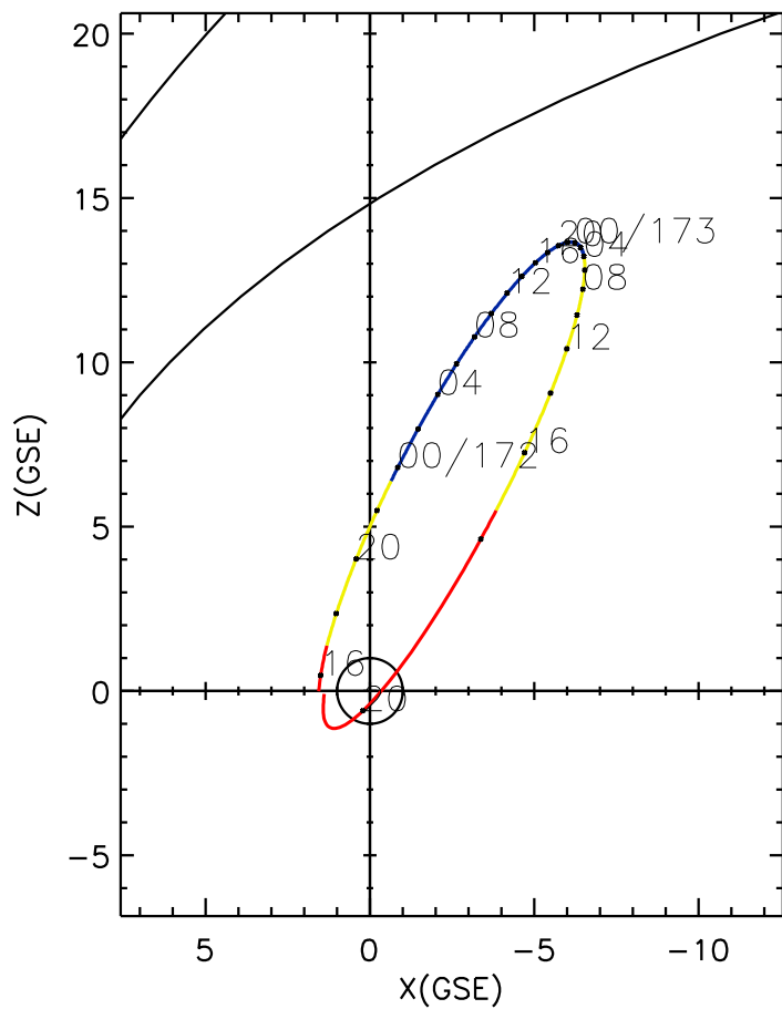
CLUSTER 2 orbit 2024 171 (06/19) 15:31 UT to 2024 173 (06/21) 21:41 UT
