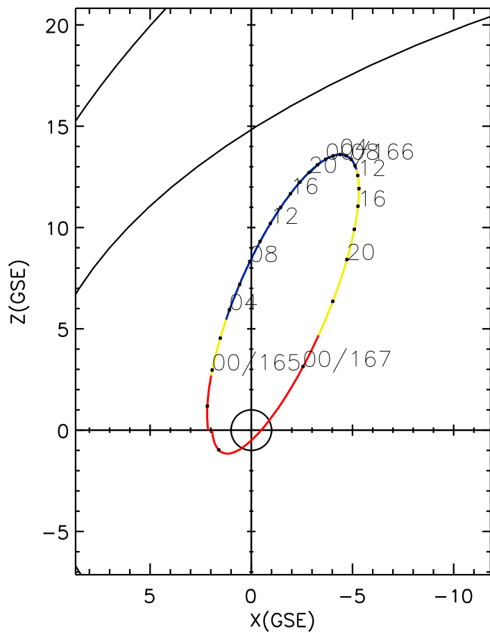
CLUSTER 2 orbit 2024 164 (06/12) 20:46 UT to 2024 167 (06/15) 03:01 UT
