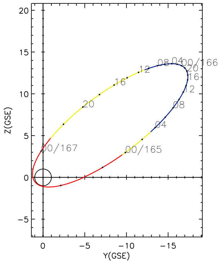
CLUSTER 2 orbit 2024 164 (06/12) 20:46 UT to 2024 167 (06/15) 03:01 UT
