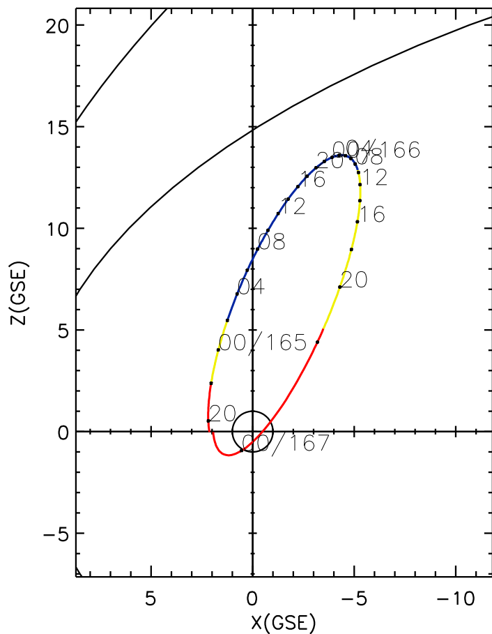
CLUSTER 2 orbit 2024 164 (06/12) 19:26 UT to 2024 167 (06/15) 01:41 UT
