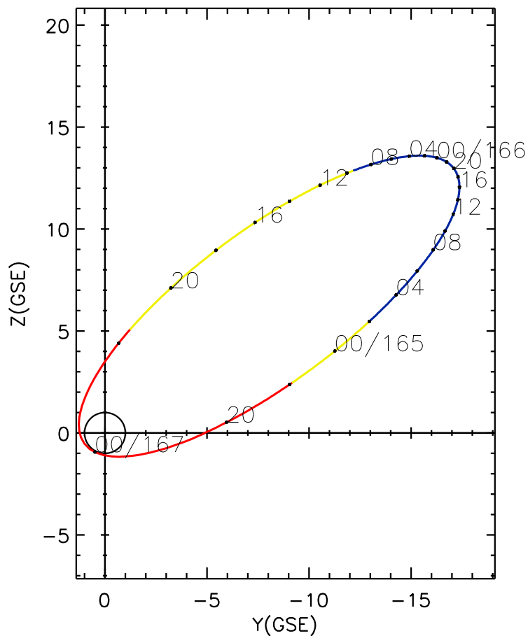
CLUSTER 2 orbit 2024 164 (06/12) 19:26 UT to 2024 167 (06/15) 01:41 UT
