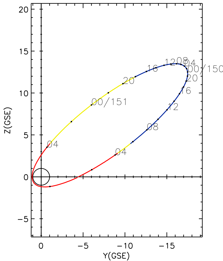
CLUSTER 2 orbit 2024 149 (05/28) 01:06 UT to 2024 151 (05/30) 07:16 UT
