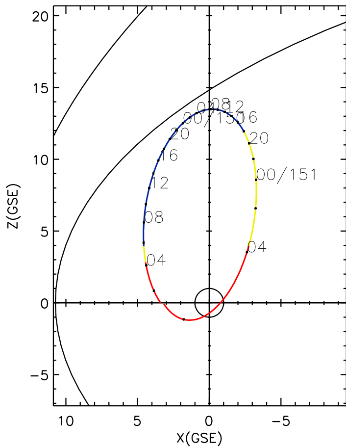
CLUSTER 2 orbit 2024 149 (05/28) 01:06 UT to 2024 151 (05/30) 07:16 UT
