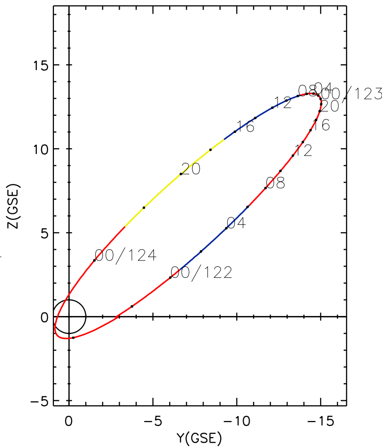
CLUSTER 2 orbit 2024 121 (04/30) 21:16 UT to 2024 124 (05/03) 03:31 UT
