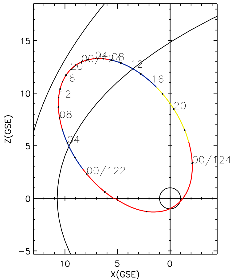
CLUSTER 2 orbit 2024 121 (04/30) 21:16 UT to 2024 124 (05/03) 03:31 UT
