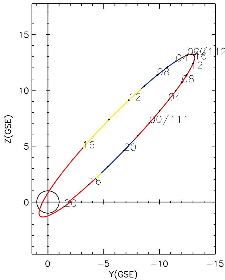
CLUSTER 2 orbit 2024 110 (04/19) 14:11 UT to 2024 112 (04/21) 20:26 UT
