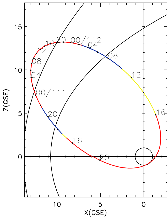
CLUSTER 2 orbit 2024 110 (04/19) 14:11 UT to 2024 112 (04/21) 20:26 UT
