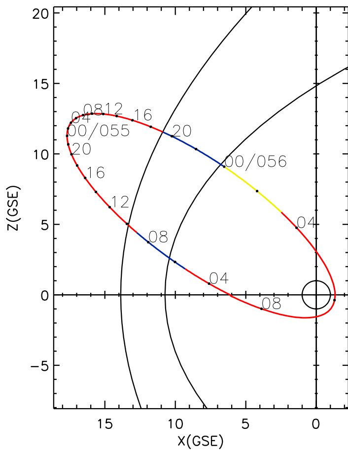
CLUSTER 2 orbit 2024 054 (02/23) 02:56 UT to 2024 056 (02/25) 09:11 UT
