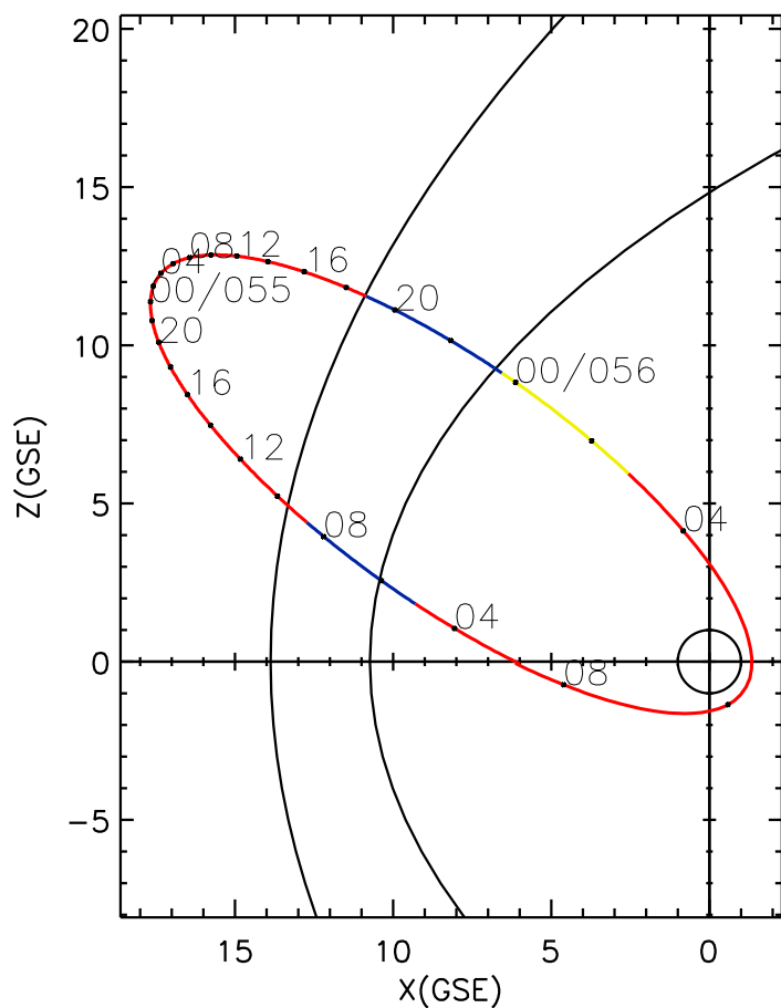
CLUSTER 2 orbit 2024 054 (02/23) 02:36 UT to 2024 056 (02/25) 08:51 UT
