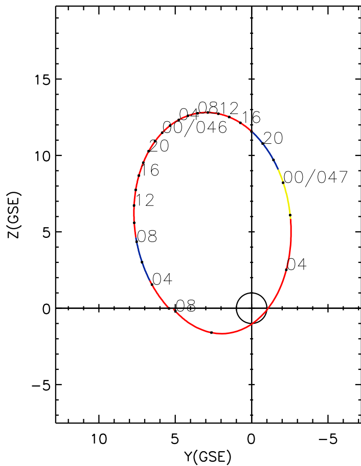
CLUSTER 2 orbit 2024 045 (02/14) 01:56 UT to 2024 047 (02/16) 08:11 UT
