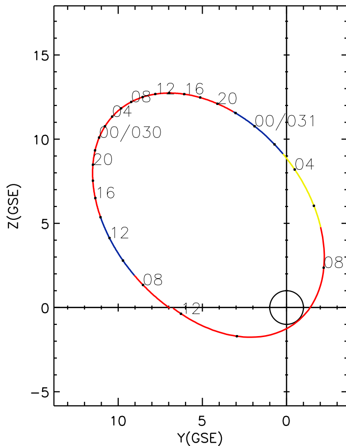
CLUSTER 2 orbit 2024 029 (01/29) 06:11 UT to 2024 031 (01/31) 12:26 UT
