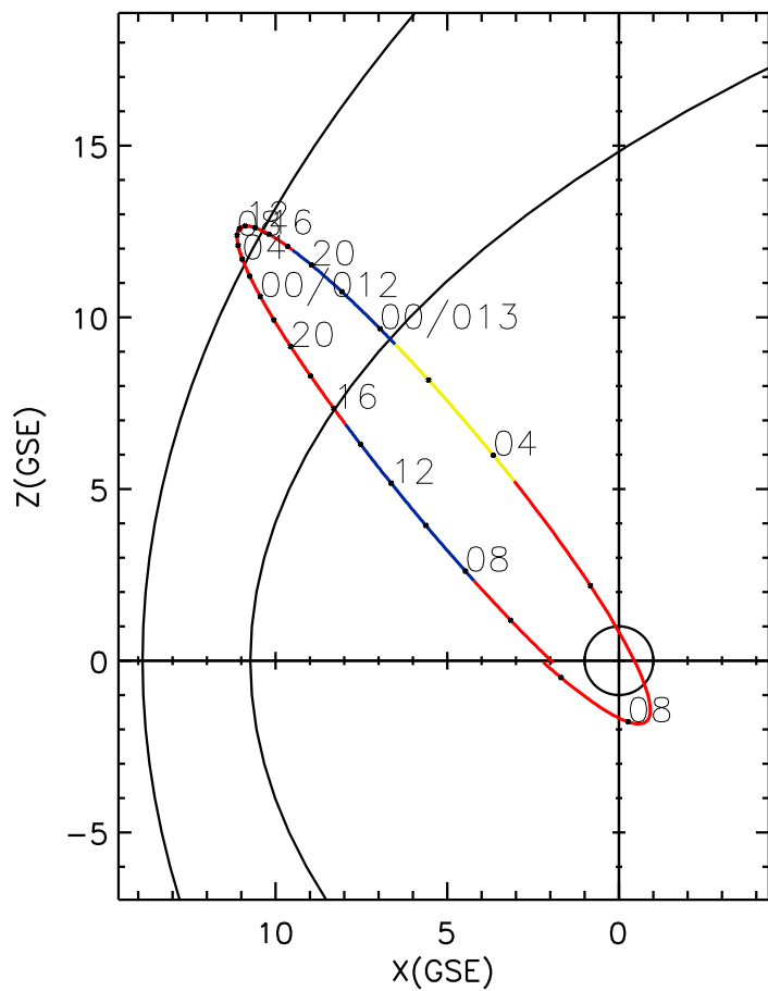
CLUSTER 2 orbit 2024 011 (01/11) 04:21 UT to 2024 013 (01/13) 10:36 UT
