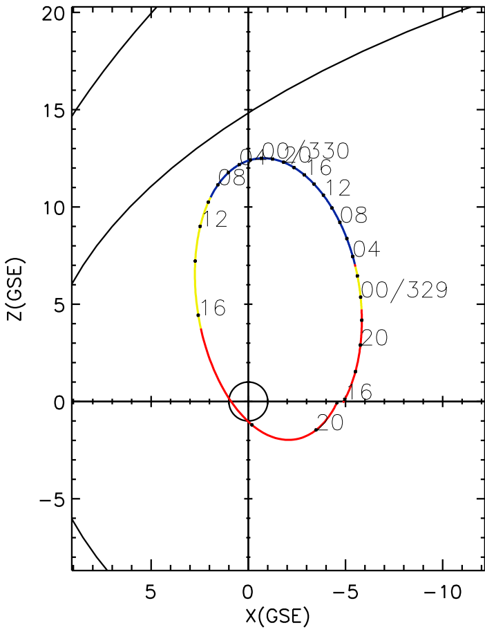
CLUSTER 2 orbit 2023 328 (11/24) 15:46 UT to 2023 330 (11/26) 22:01 UT
