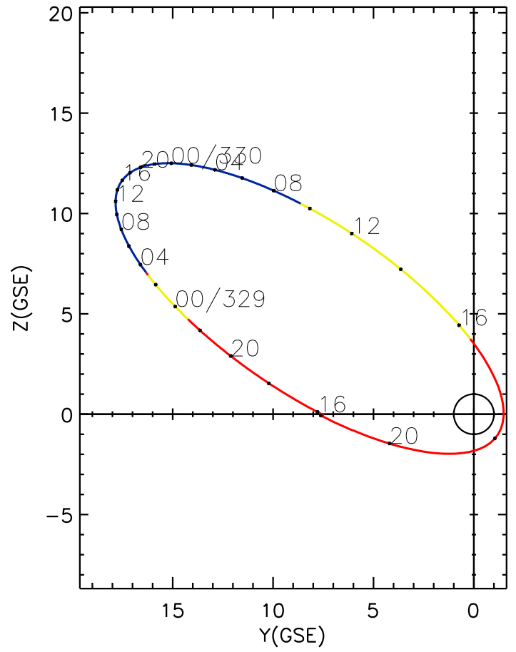
CLUSTER 2 orbit 2023 328 (11/24) 15:46 UT to 2023 330 (11/26) 22:01 UT
