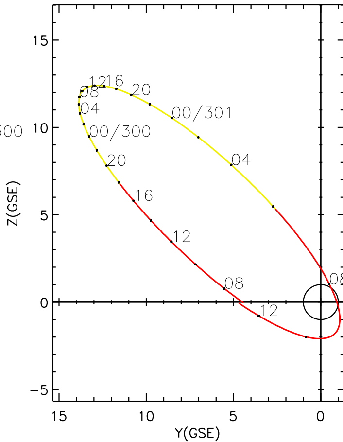
CLUSTER 2 orbit 2023 299 (10/26) 06:51 UT to 2023 301 (10/28) 13:01 UT
