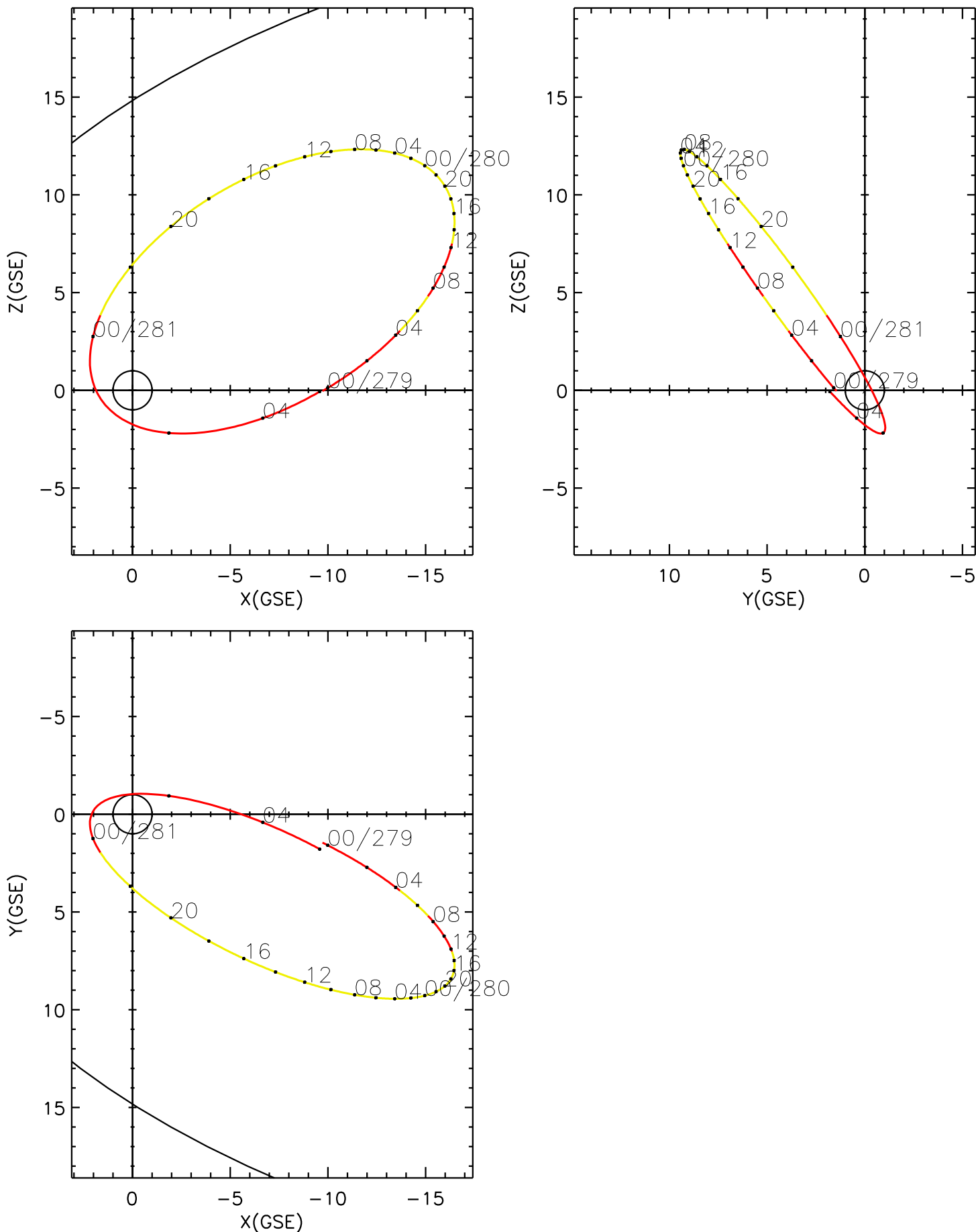
CLUSTER 2 orbit 2023 278 (10/05) 23:46 UT to 2023 281 (10/08) 06:01 UT
